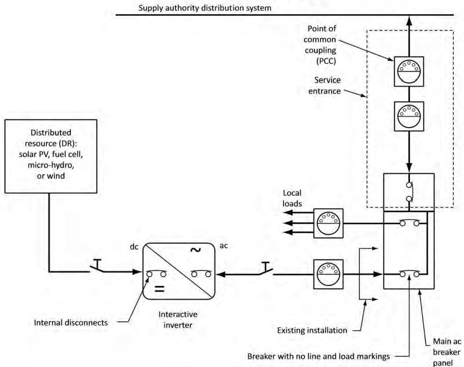
Figure B64-1 Typical renewable energy system
