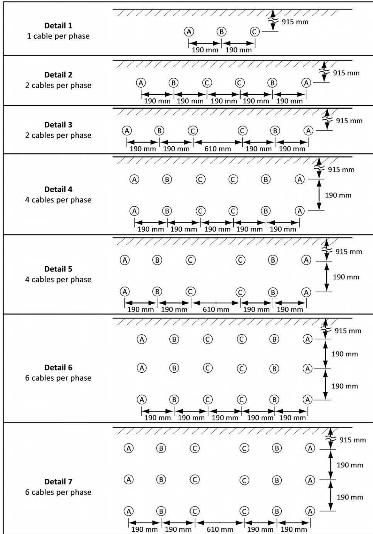
Diagram D8 Installation configurations — Direct buried
