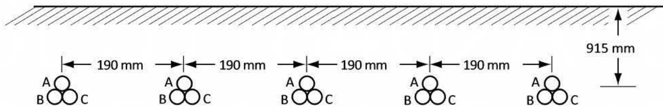
Detail 5 5 cables per phase
