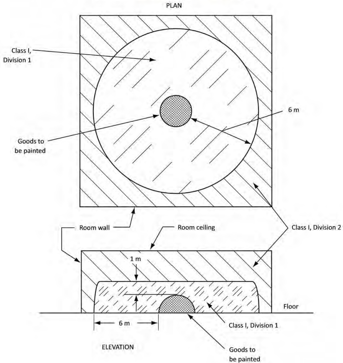
Diagram JD-5 Extent of hazardous location for spraying operations not conducted in spray booths [See Rules J20-302 1) b) and J20-302 4).]
