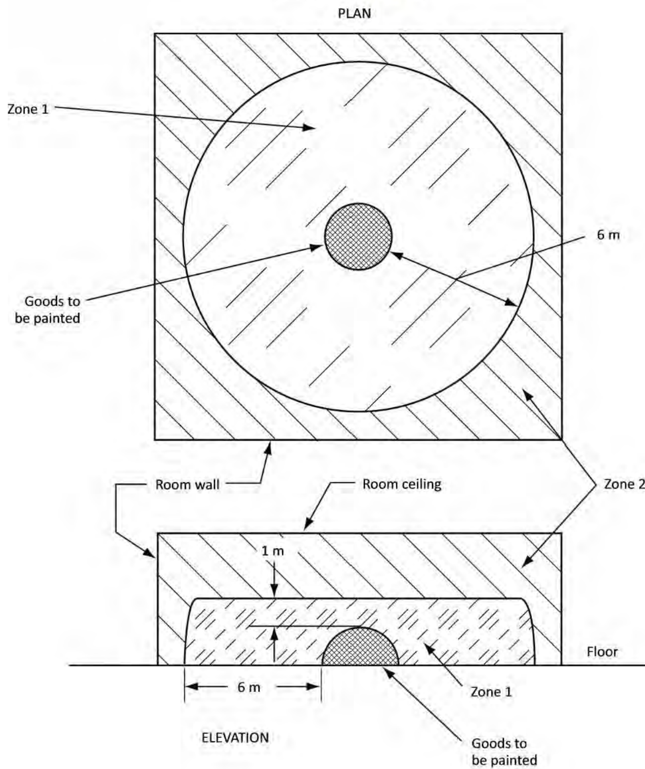
Diagram 5 Extent of hazardous location for spraying operations not conducted in spray booths (See Rule 20-302.)
