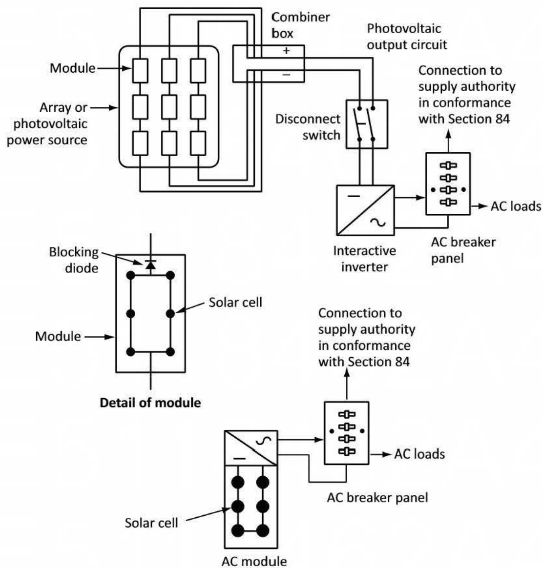
Figure B64-4 Interconnected system
