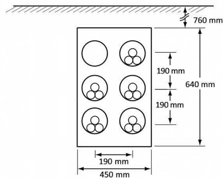
Detail 5 — 5 insulated conductors or cables per phase
