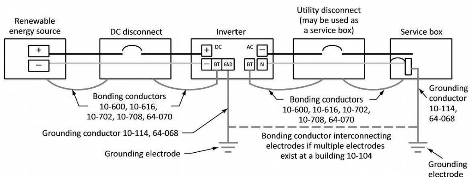
Rule 64-068 b) Grounding electrode requirements
