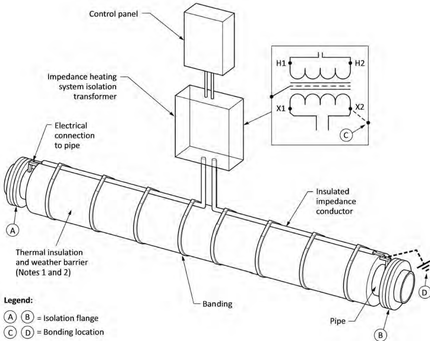
Figure B62-9 End feed system
