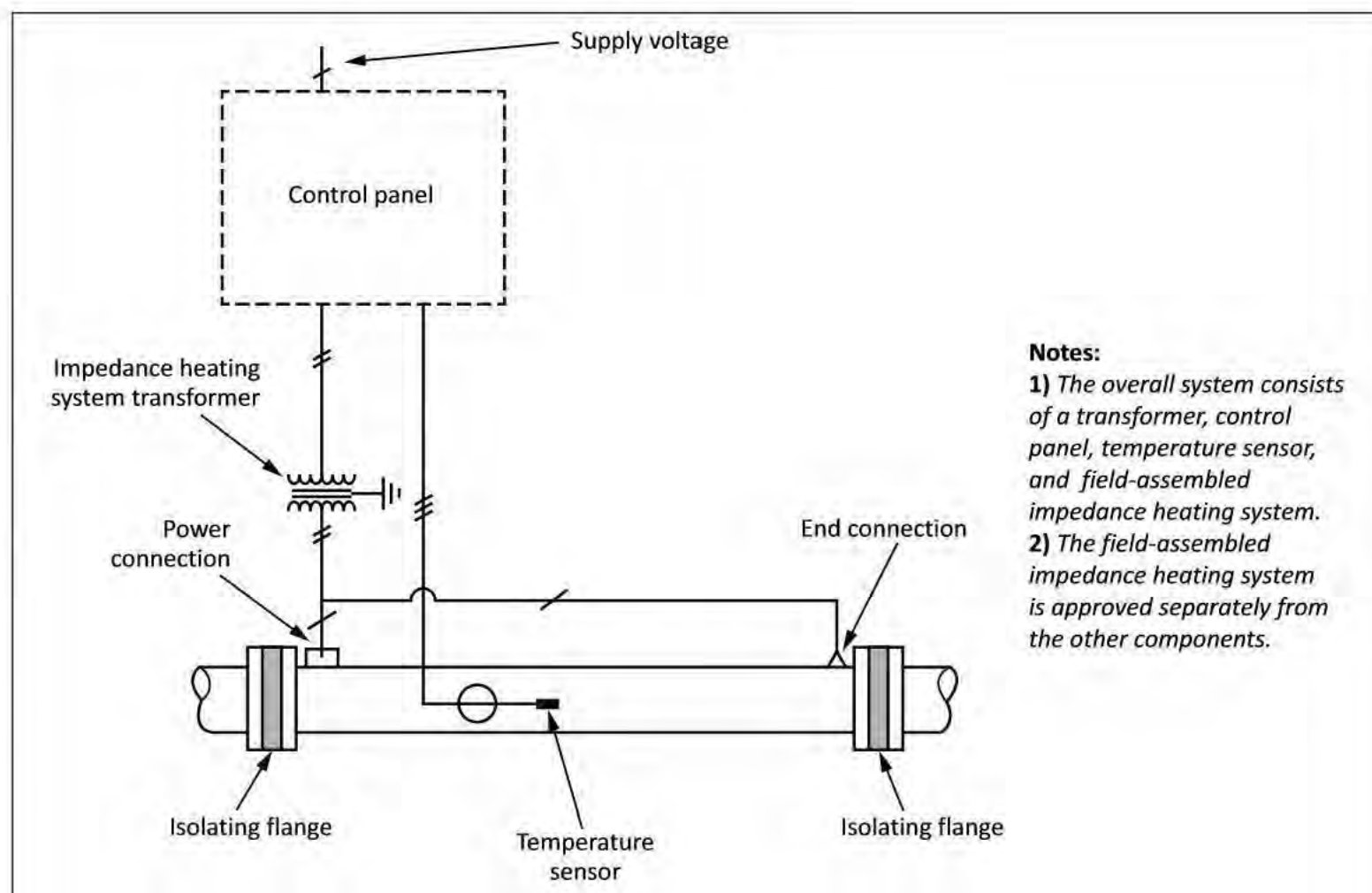
Figure B62-7 Typical impedance heating system
