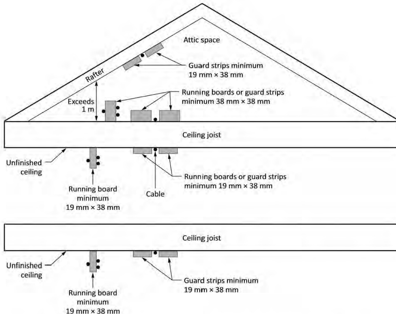
Figure B12-3 Running boards and guard strips
