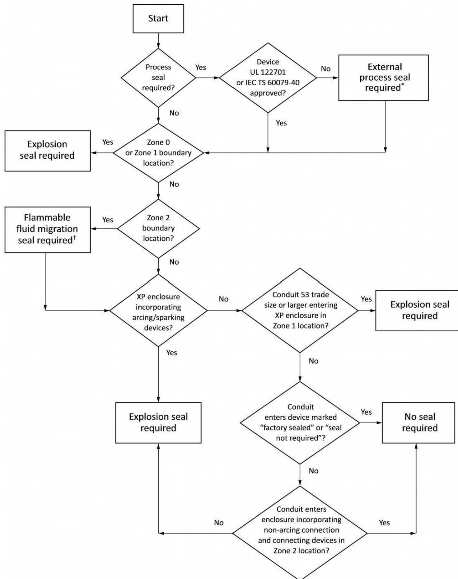
Figure JB18-3 Flow chart for seals selection using conduits
