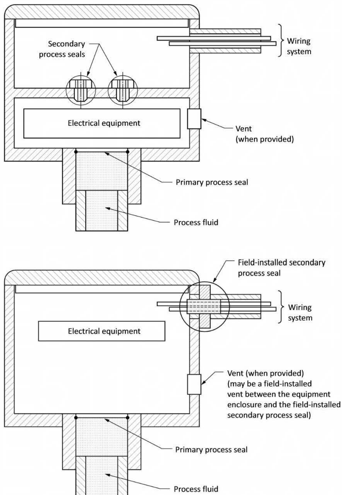
Figure B18-1 Process sealing
