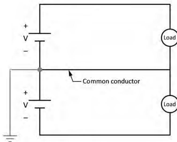
Figure B10-2 Series dc sources (bipolar)
