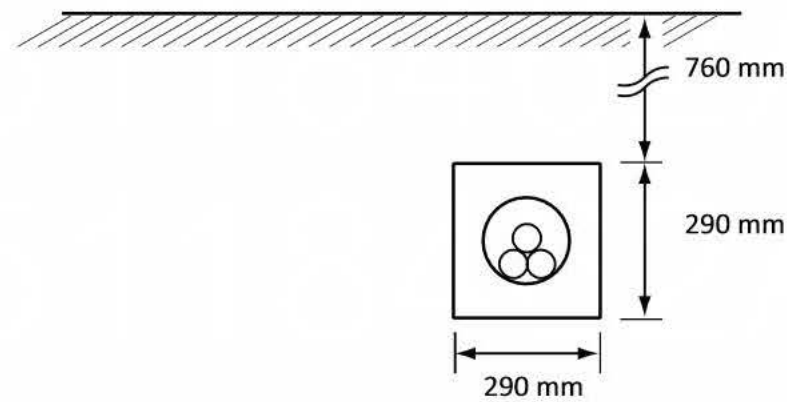
Detail 1 — 1 insulated conductor or cable per phase
