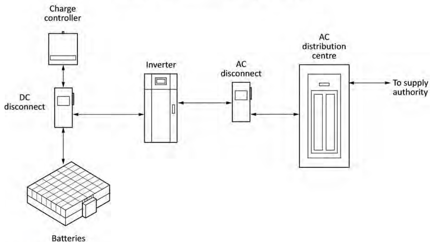
Figure B64-10 Field-assembled energy storage
