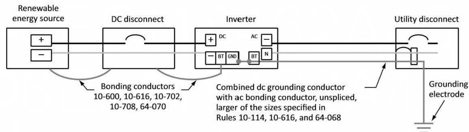
Rule 64-068 c) Grounding electrode requirements
