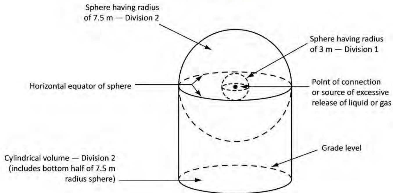
Diagram JD-7 Extent of hazardous location for tank vehicle and tank car loading and unloading (See Part B of Table JT-63.)
