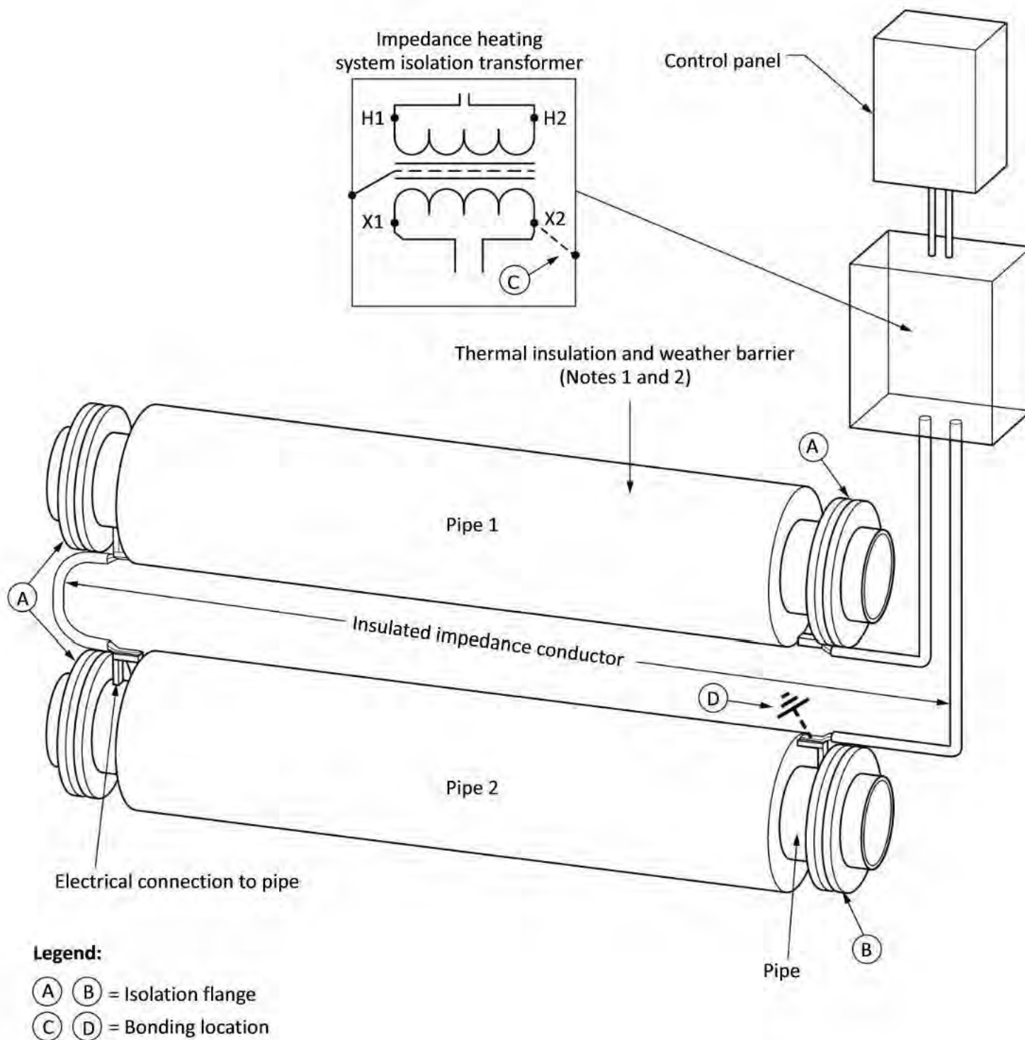
Figure B62-10 Dual line and end feed system
