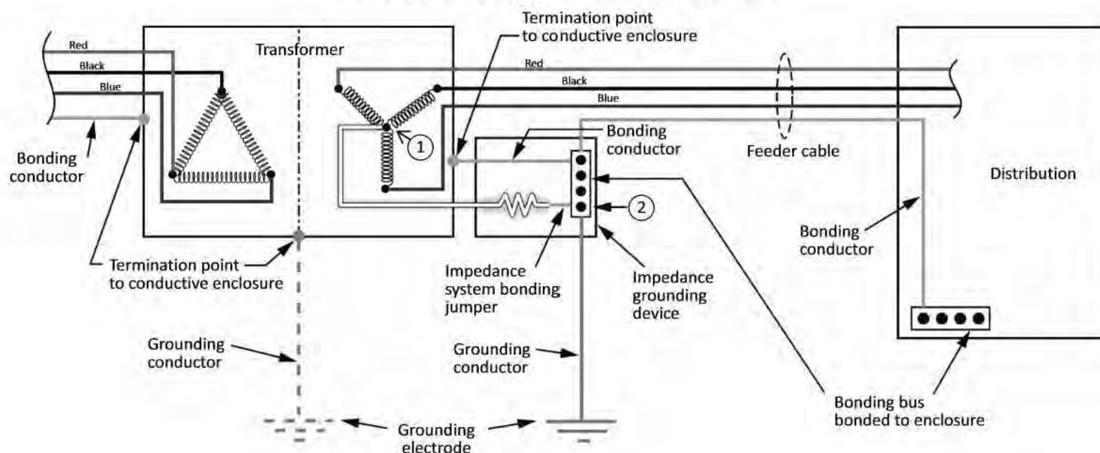
Figure B10-12 Impedance grounded system
