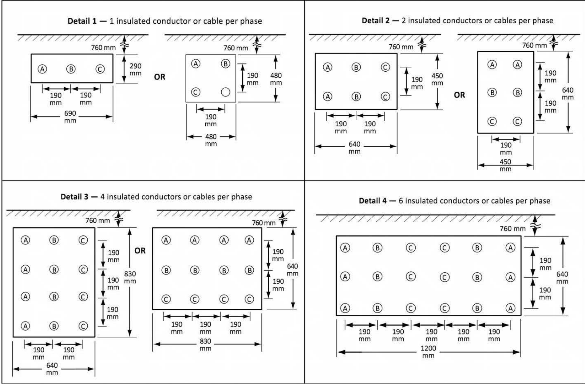
Diagram D9 Installation configurations — Conduit or raceway
