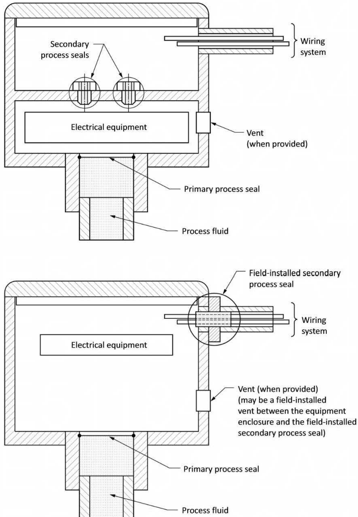
Figure JB18-1 Process sealing
