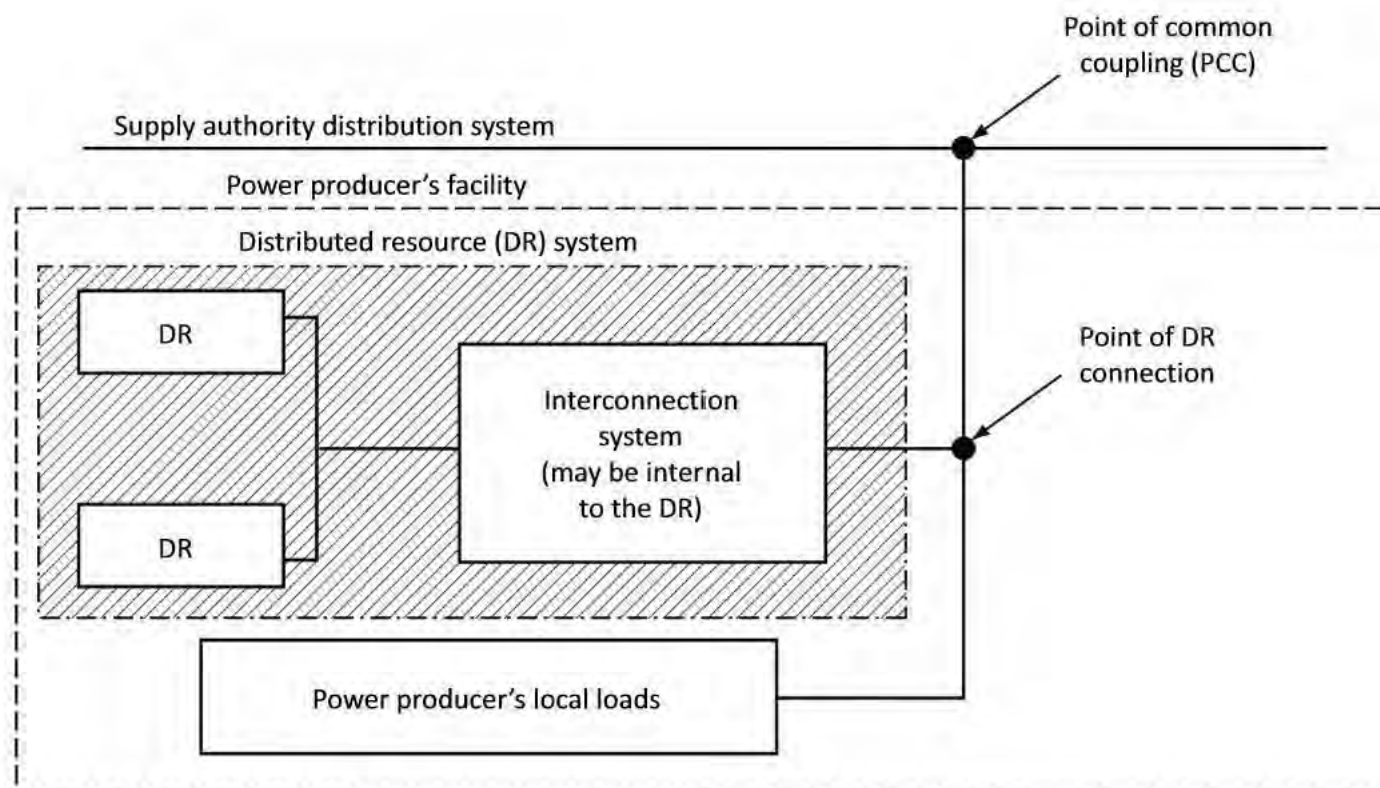
Figure B64-6 Point of common coupling
