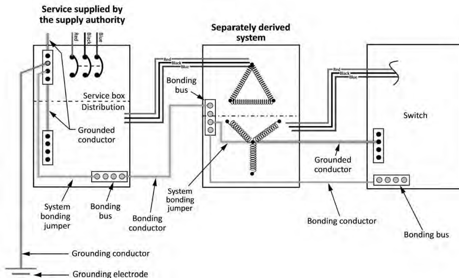
Figure B10-11 Grounding alternative for a separately derived system operating at 750 V or less
