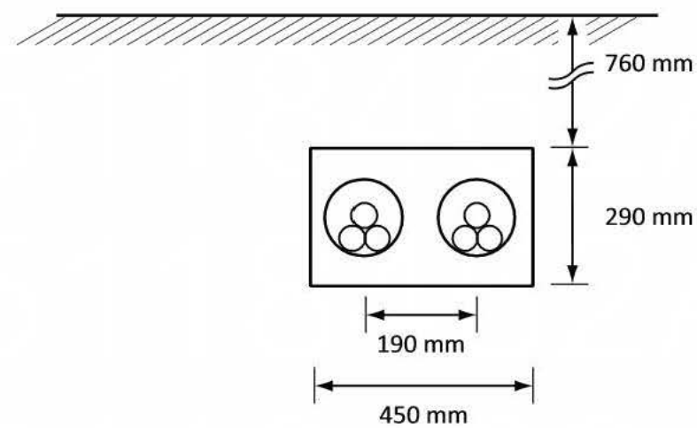
Detail 2 — 2 insulated conductors or cables per phase
