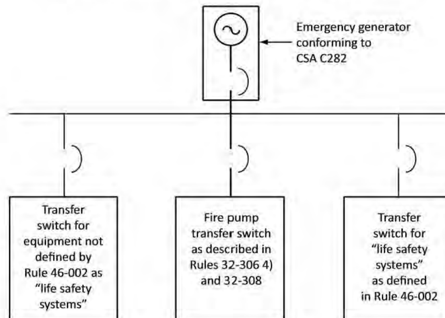
Figure B46-1 Connections to an emergency generator
