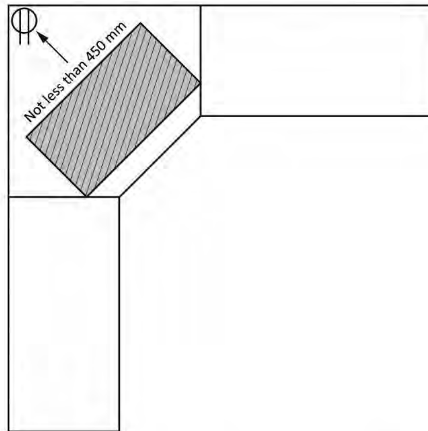
Figure B26-2 Receptacles behind sinks
