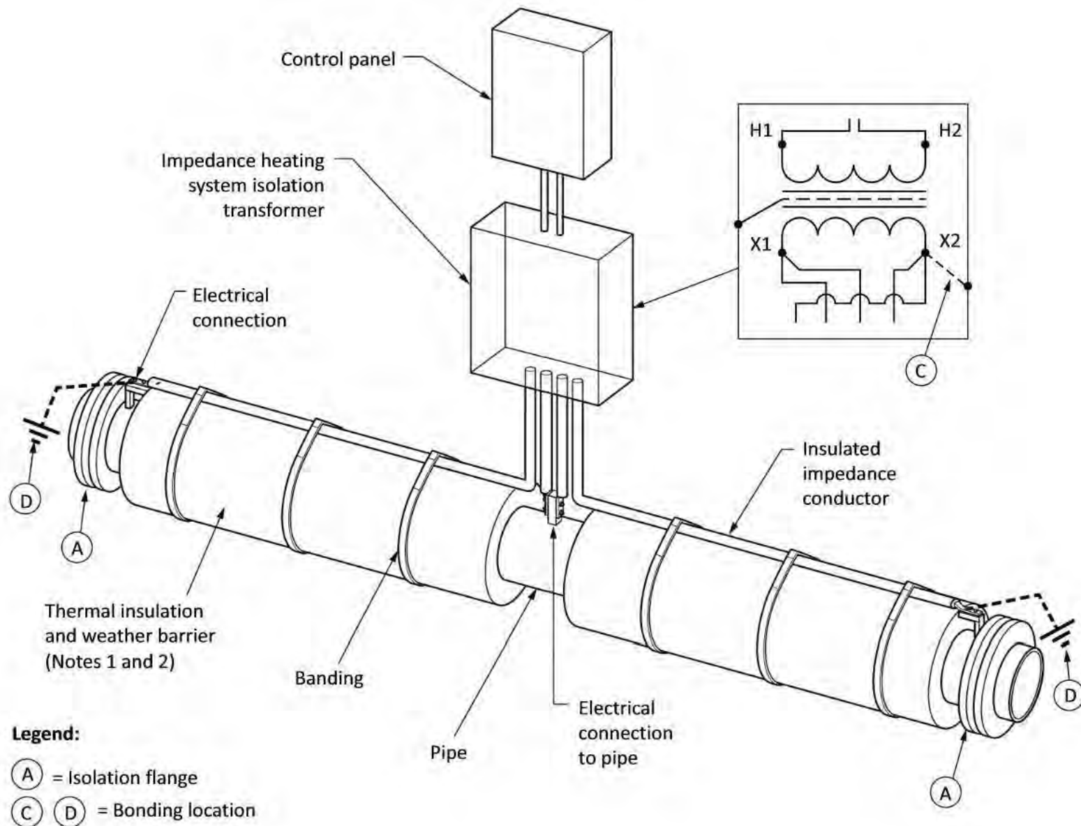
Figure B62-8 Midpoint feed system
