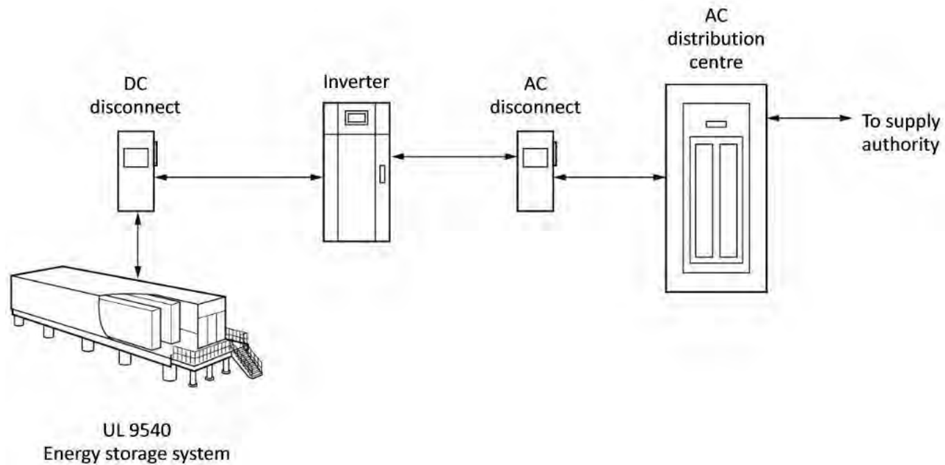
Figure B64-9 Self-contained energy storage
