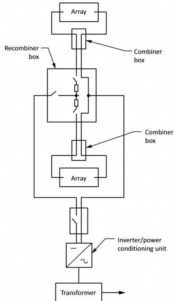
Figure B64-5 Large interconnected system
