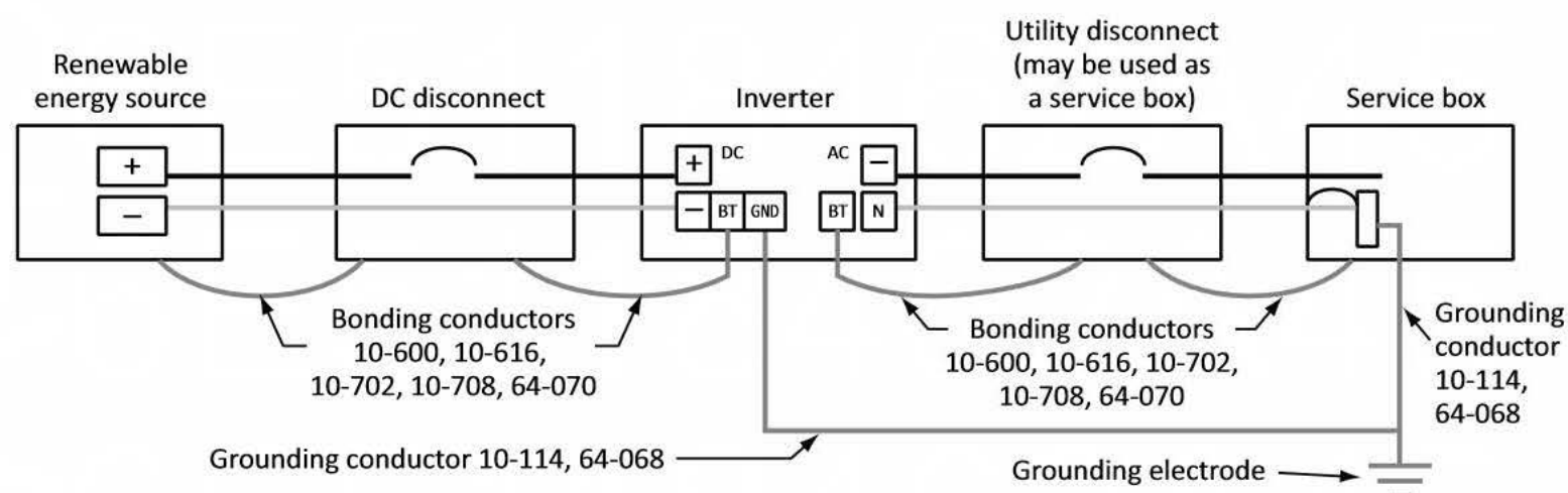
Rule 64-068 a) Grounding electrode requirements
