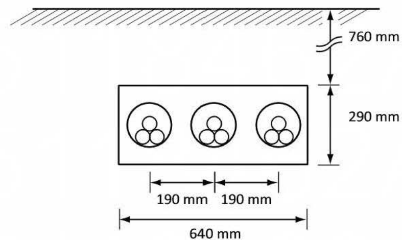
Detail 3 — 3 insulated conductors or cables per phase
