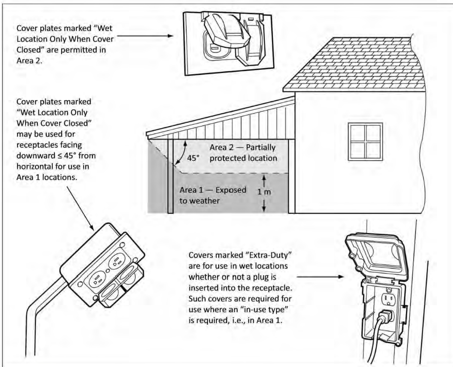
Figure B26-3 Covers for receptacles located outdoors
