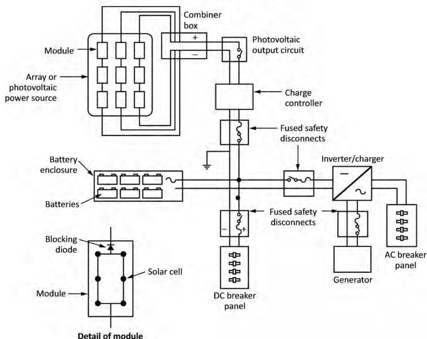
Figure B64-3 Stand-alone system
