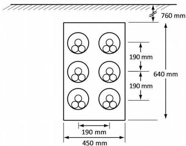
Detail 6 — 6 insulated conductors or cables per phase
