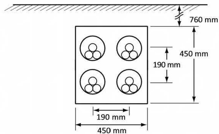
Detail 4 — 4 insulated conductors or cables per phase
