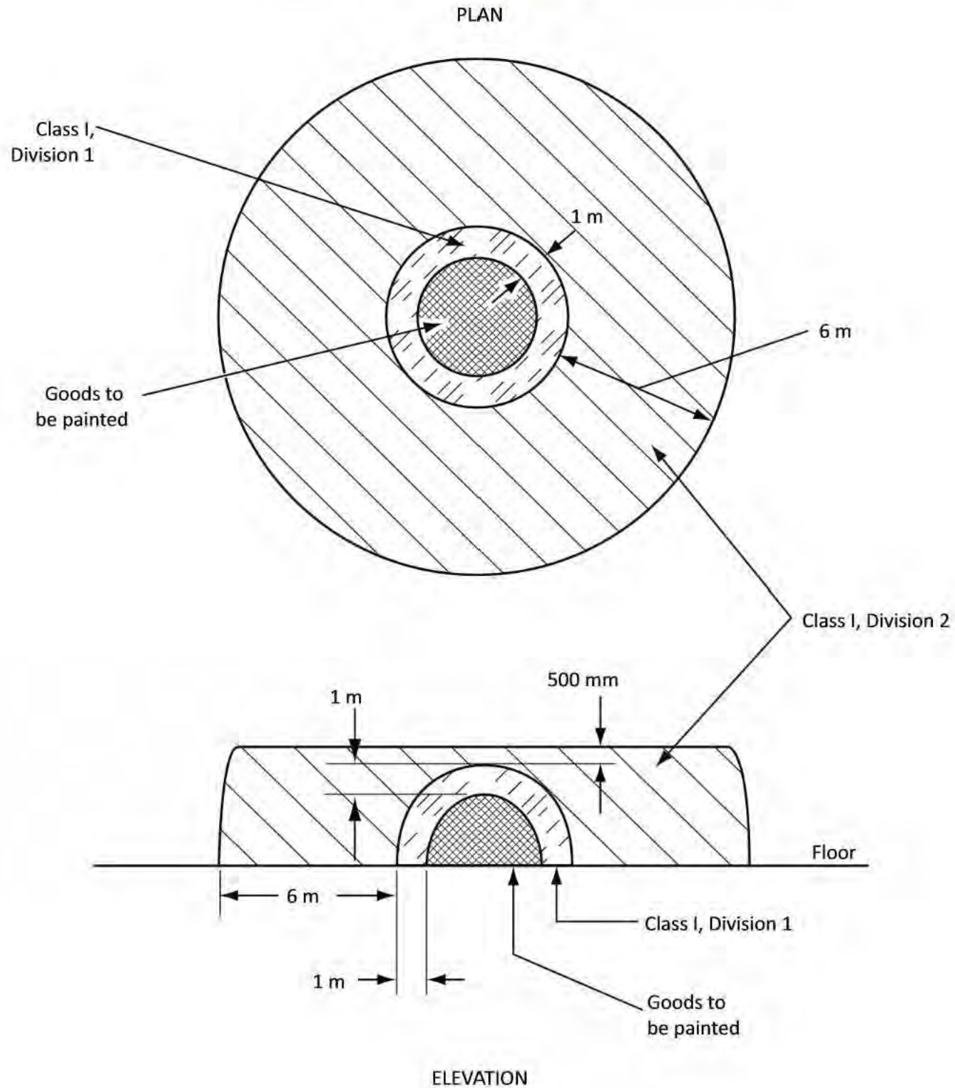
Diagram JD-6 Extent of hazardous location for spraying operations not conducted in spray booths — Ventilation system interlocked [See Rule J20-302 7).]
